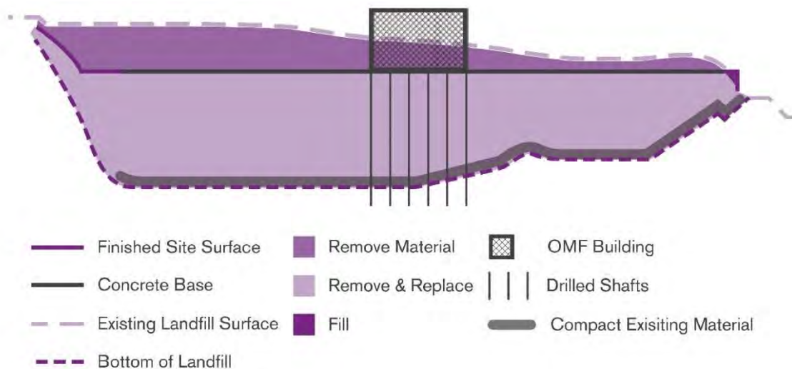
Figure 2.3-8 Hybrid Subsurface Construction Design Option Cross Section
