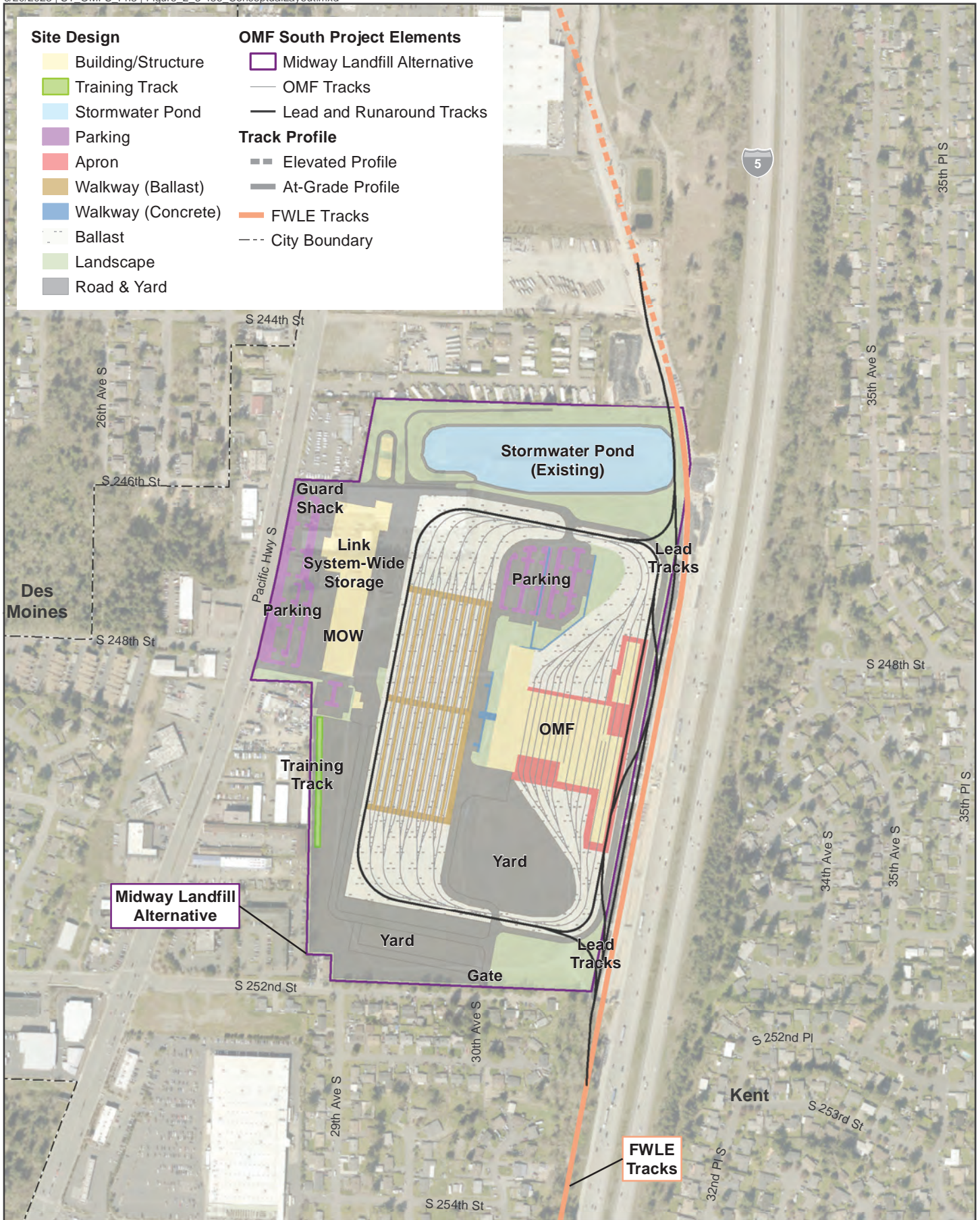
FIGURE 2.3-6 Conceptual Layout Midway Landfill Alternative OMF South
