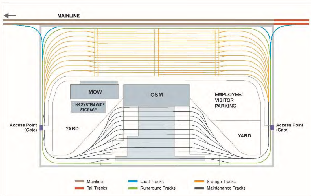
Figure 2.1-3 Typical OMF Schematic
