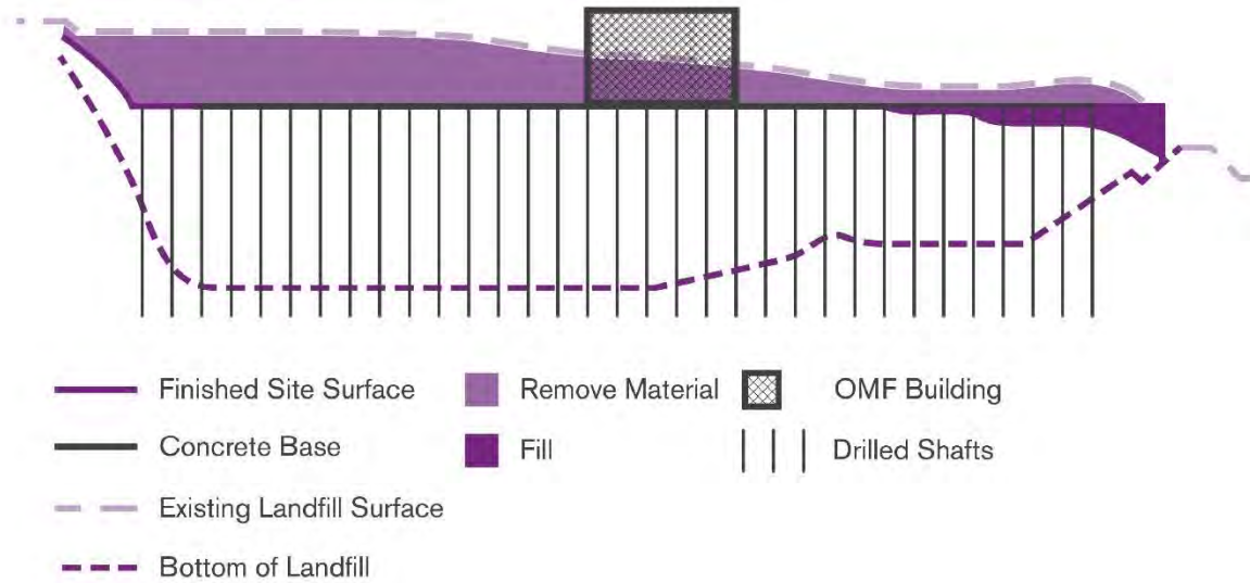
Figure 2.3-7 Platform Subsurface Construction Design Option Cross Section
