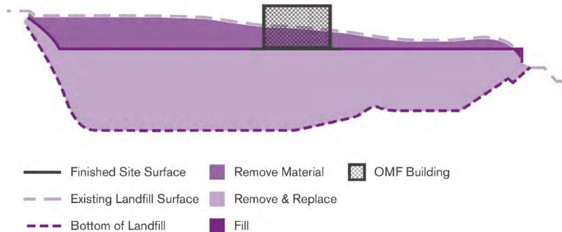
Figure 2.3-9 Full Excavation Subsurface Construction Design Option Cross Section
