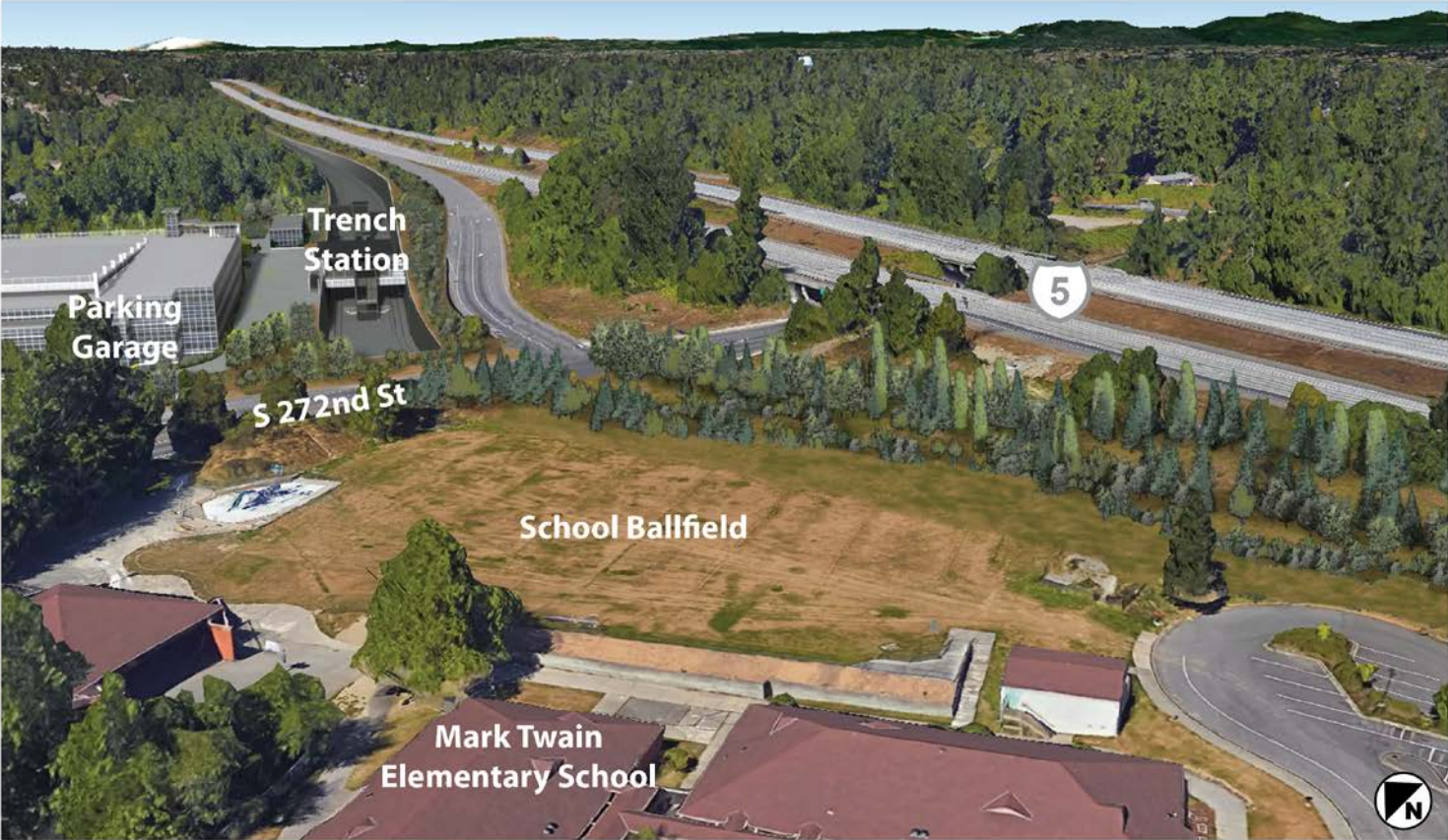
Trench Option Preferred Alternative
